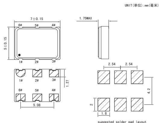
Pin Connection
